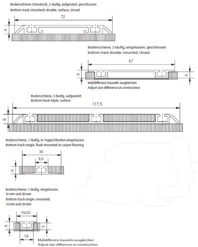
OVERVIEW OF BOTTOM TRACK – 42 SERIES
