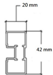
STILE – S1500 SERIES
