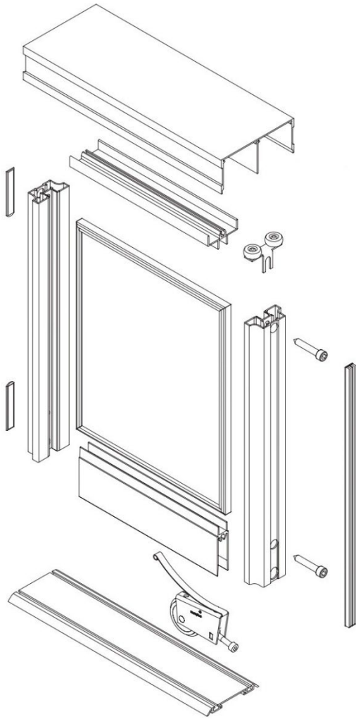
EXPLODED DRAWING – RAUMPLUS S1500 SERIES
