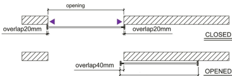
SLIDING DOOR OVERLAPPING
