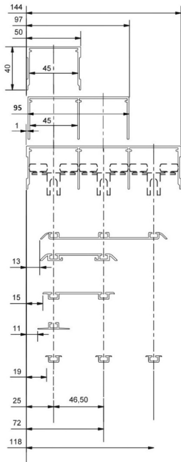
POSITION OF BOTTOM TRACK – 42 SERIES [S1500/S3000]
