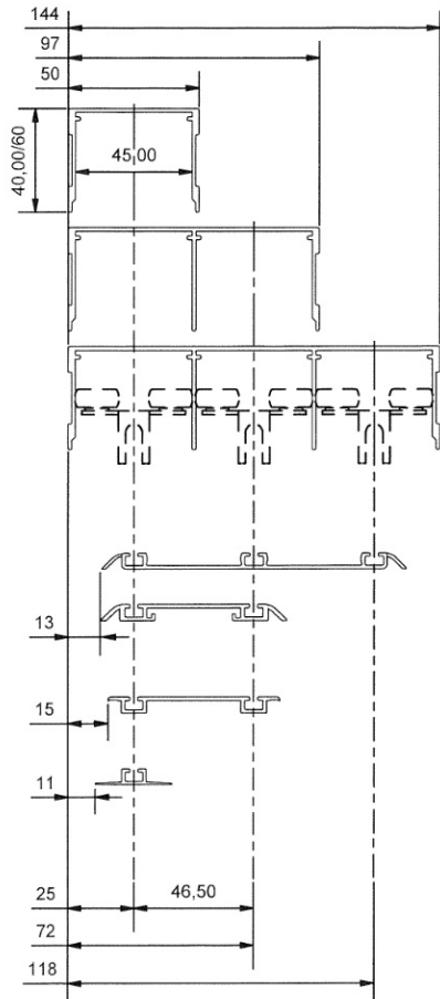
POSITION OF BOTTOM TRACK-42 SERIES [S1500/S3000]
