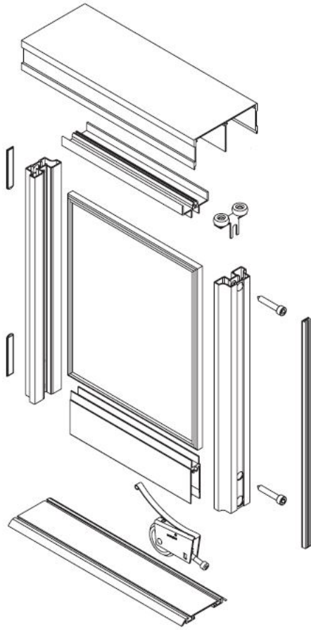
EXPLODED DRAWING – RAUMPLUS S1500 SERIES
