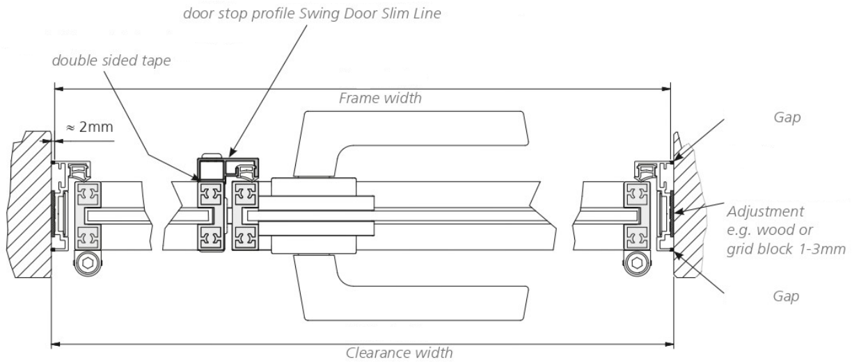
HORIZONTAL SECTION – SWING SLIM DOUBLE
