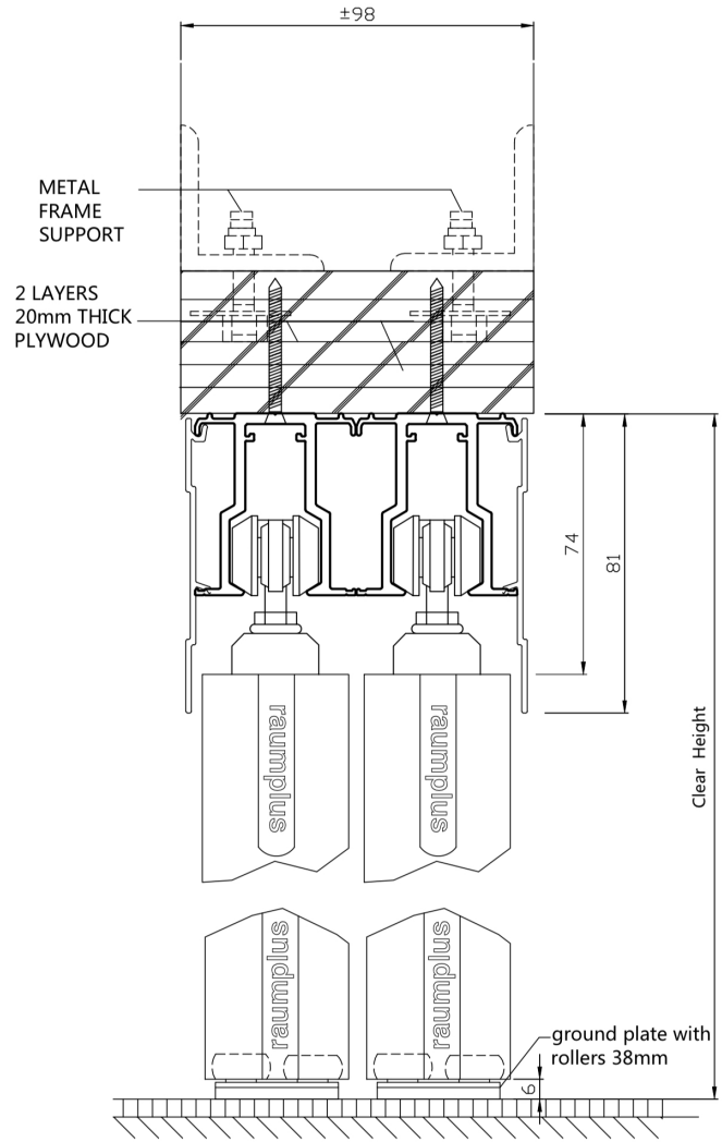
STANDARD CEILING MOUNT PROVISION – S42 AIR SERIES
