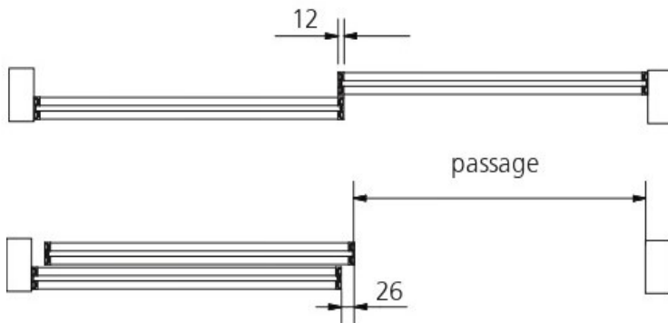
2-SLIDING DOOR OVERLAPPING
