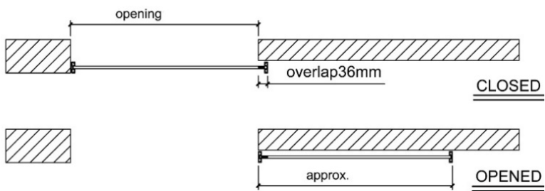
1-SLIDING DOOR OVERLAPPING (FLUSH)
