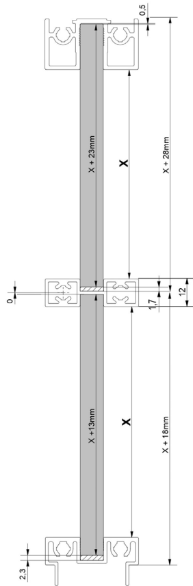
DETAIL SECTION – S1200 DIVIDING RAILS
