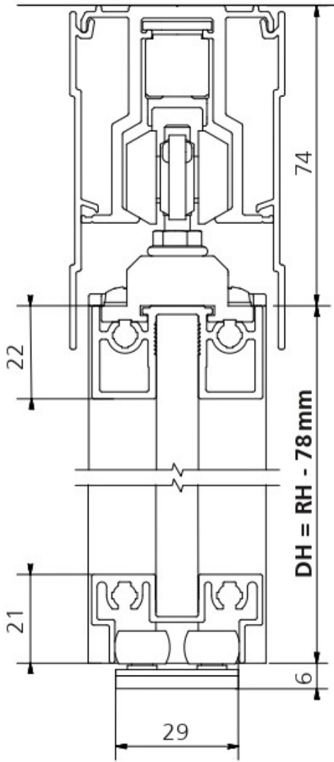
VERTICAL SECTION [S1200_AIR_SDB]
