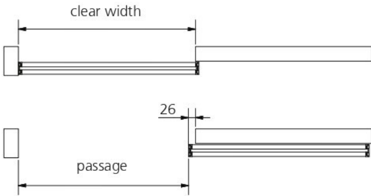
1-SLIDING DOOR OVERLAPPING
